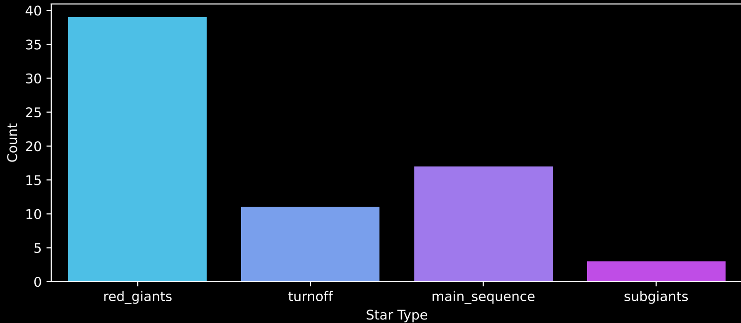
GALAH DR4 Field: [-2] Count plot of Star Type
