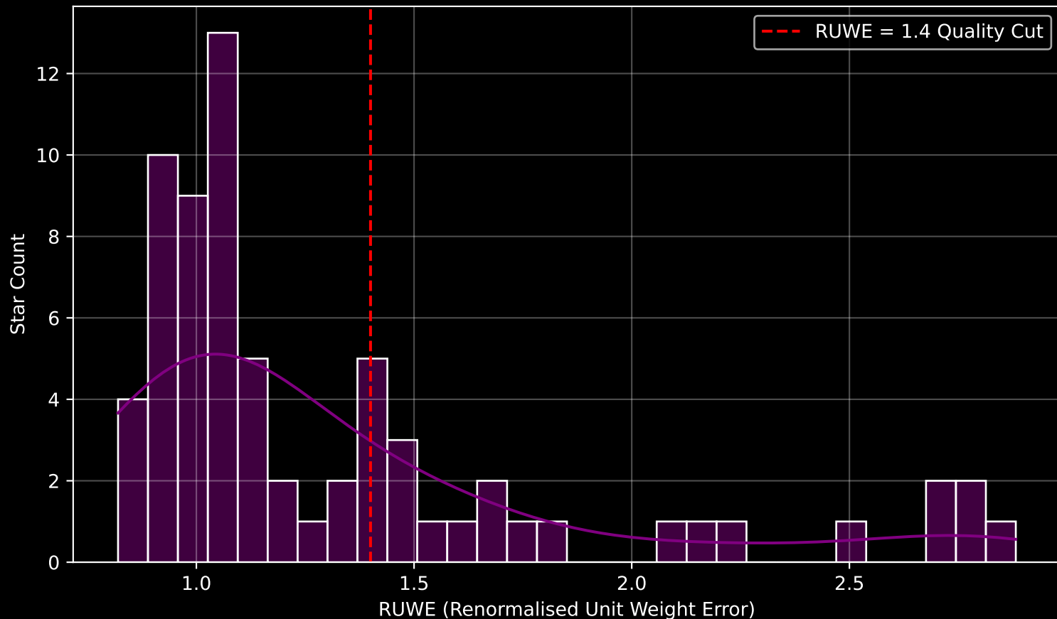
GALAH DR4 Field [-2] RUWE Distribution (n= 69)
