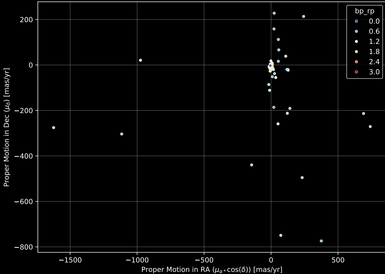
GALAH DR4 Field: [-2] Proper Motion Diagram (n= 70)
